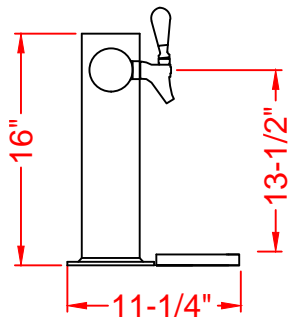
PE-TTT-8 SIDE VIEW
