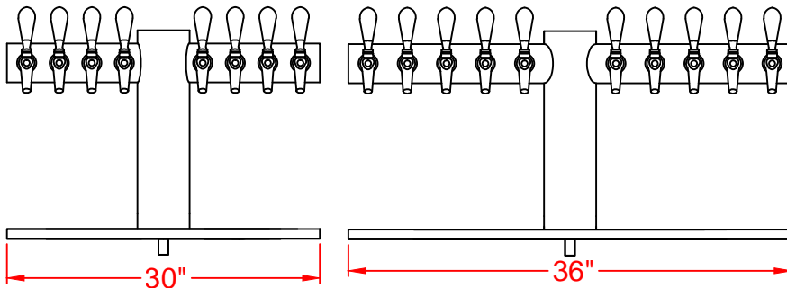
PE-TTT-8 FRONT VIEW
