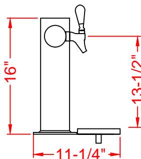
PE-TTT-10 SIDE VIEW
