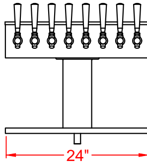
PE-8TT FRONT VIEW PE-7TT SAME DIMENSIONS
