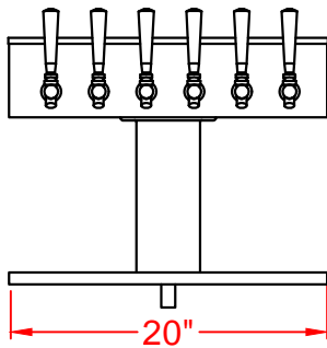
PE-6TT FRONT VIEW PE-5TT SAME DIMENSIONS
