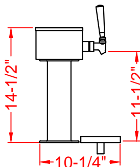
PE-8TT SIDE VIEW PE-7TT SAME DIMENSIONS
