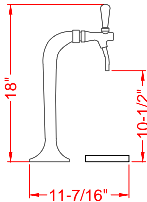
MBT-2 SIDE VIEW
