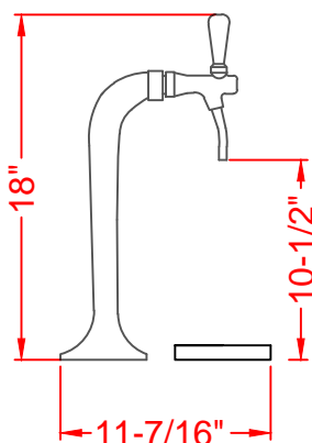
MBT-1 SIDE VIEW
