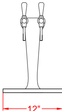
MBT-2 FRONT VIEW
