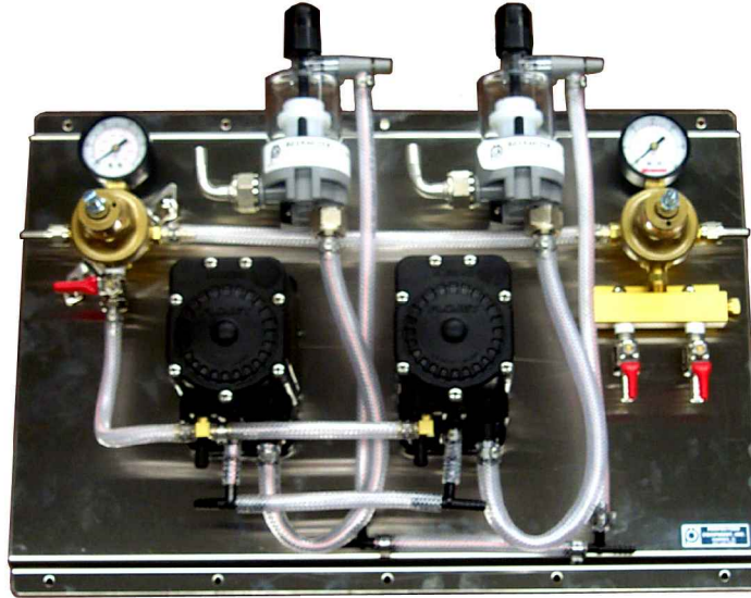
Shown Pump Panel GRP-2
