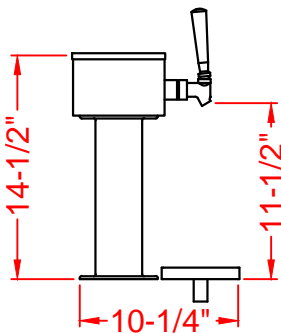
PE-3TT SIDE VIEW
