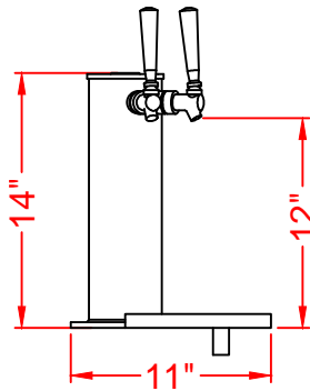
CT-4 SIDE VIEW
