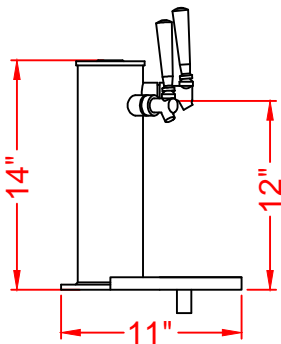
CT-3 SIDE VIEW
