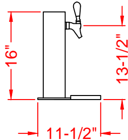
PE-GPT-10 SIDE VIEW
