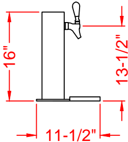
PE-GPT-8 SIDE VIEW
