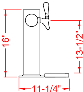
PE-TTT-8 SIDE VIEW
