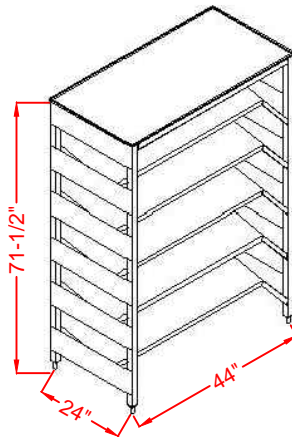
MODEL PE-15-BIB-TS Capacity (15) Bag-In-Box cartons
