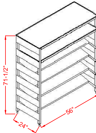
MODEL PE-16-BIB-2TS Capacity (16) Bag-In-Box cartons Additional top shelf for air compressor
