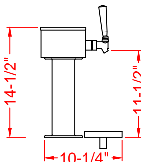
PE-4TT SIDE VIEW
