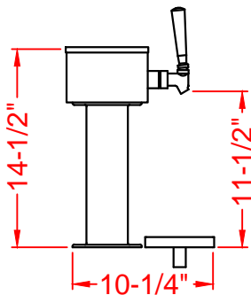
PE-3TT SIDE VIEW
